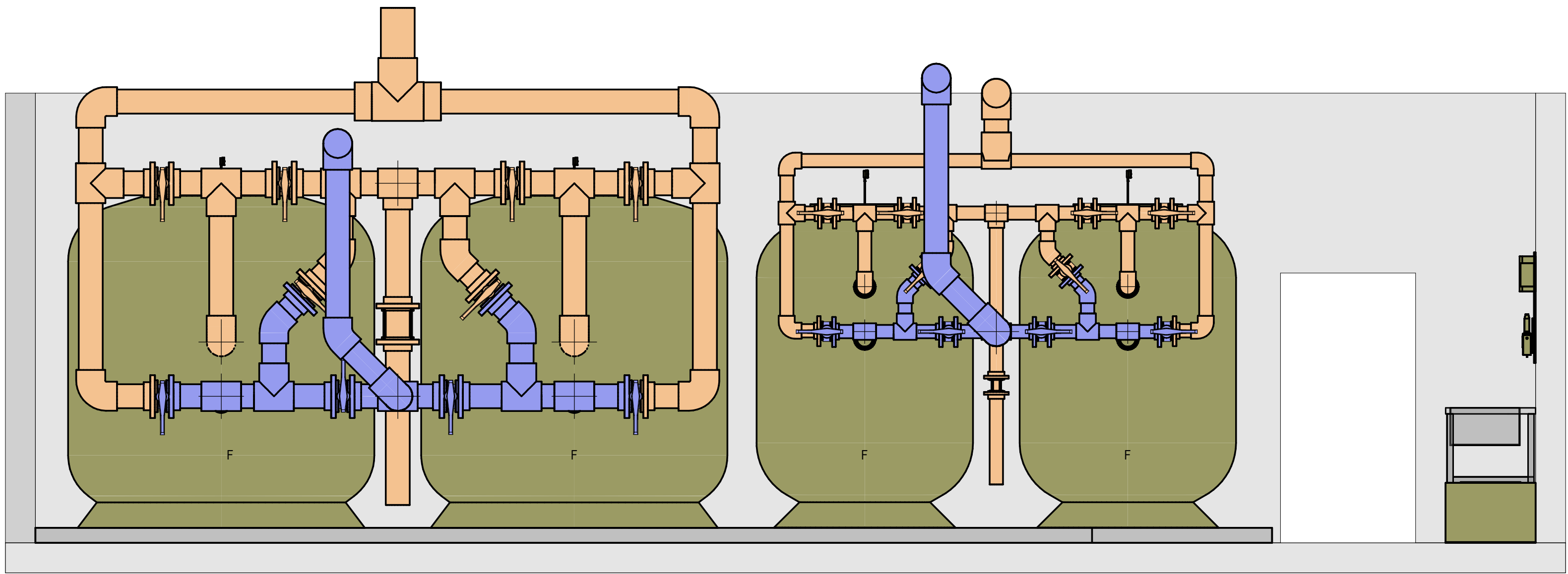
1 FILTER SECTION BWK-4001 1 : 25
