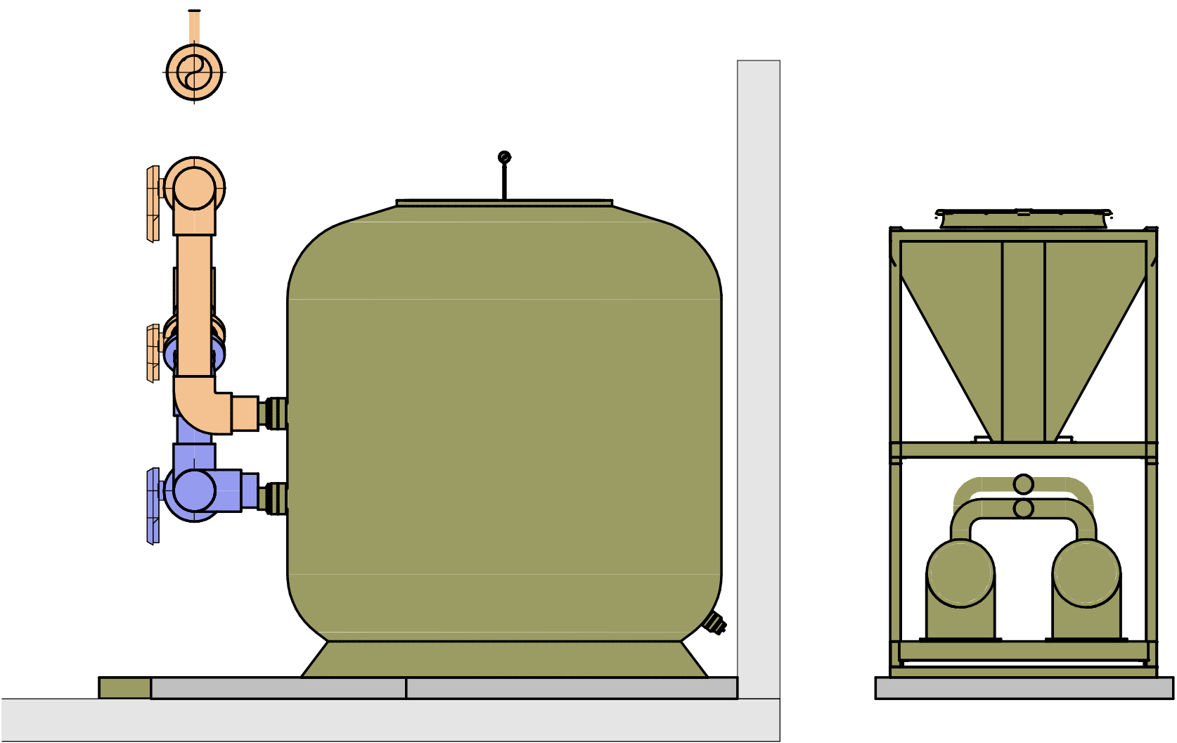
3 HEAT PUMP END SECTION BWK-4001 1 : 25
