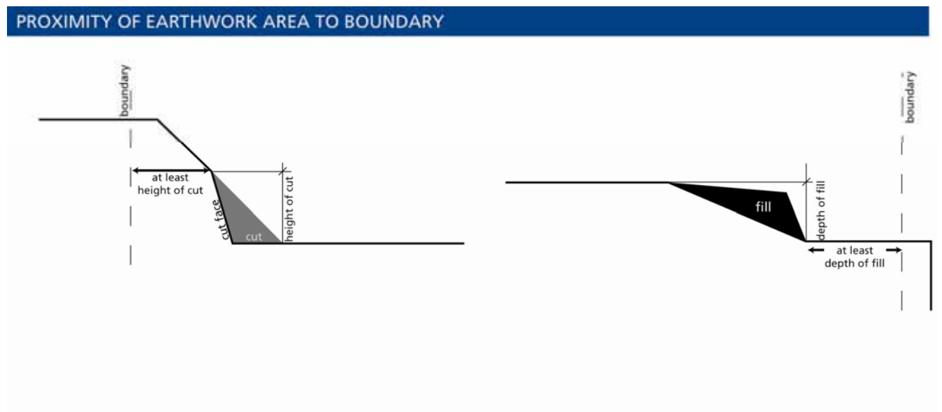
Diagram 1: Proximity of Earthwork Area to Boundary, buildings and structures
