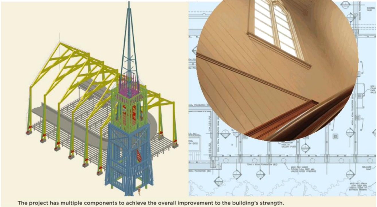
Removal, bracing behind and reinstatement of the original internal kauri cladding.
