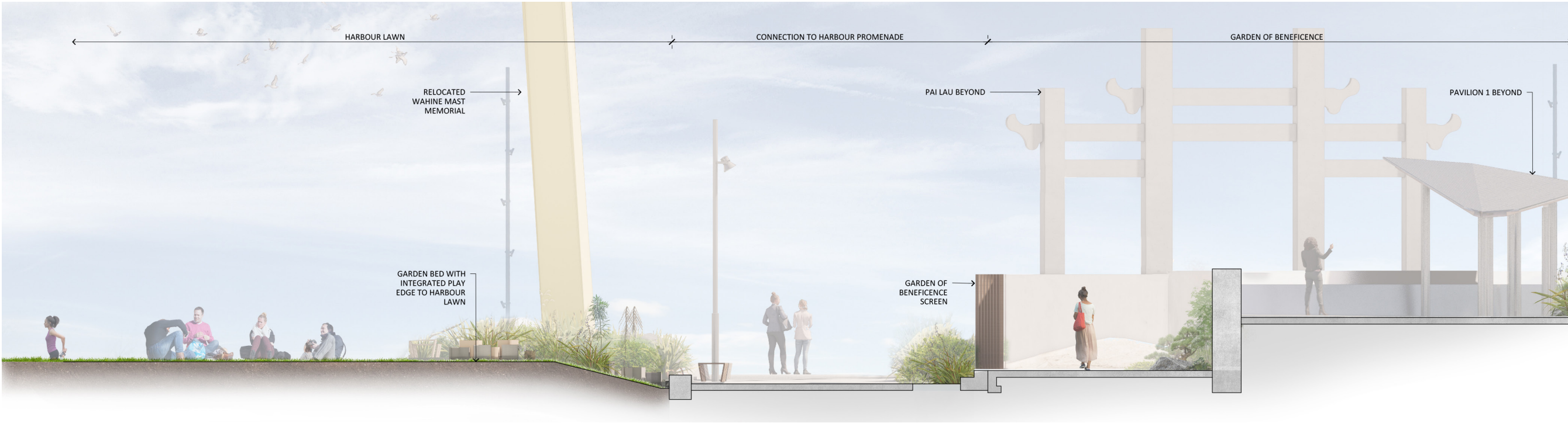
SECTION 6 (S6) - CROSS SECTION THROUGH EAST WEST PROMENADE 1:100 @ A3
