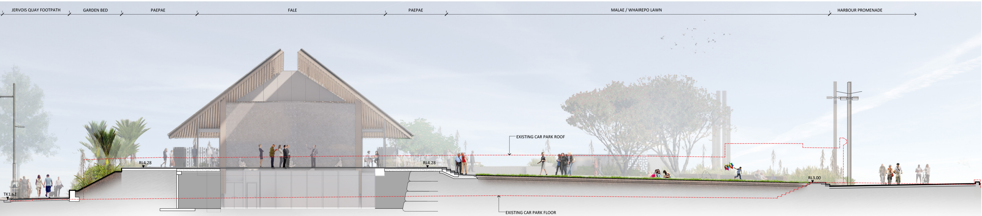
SECTION 1 (S1) - CROSS SECTION THROUGH FALE 1:200 @ A3
