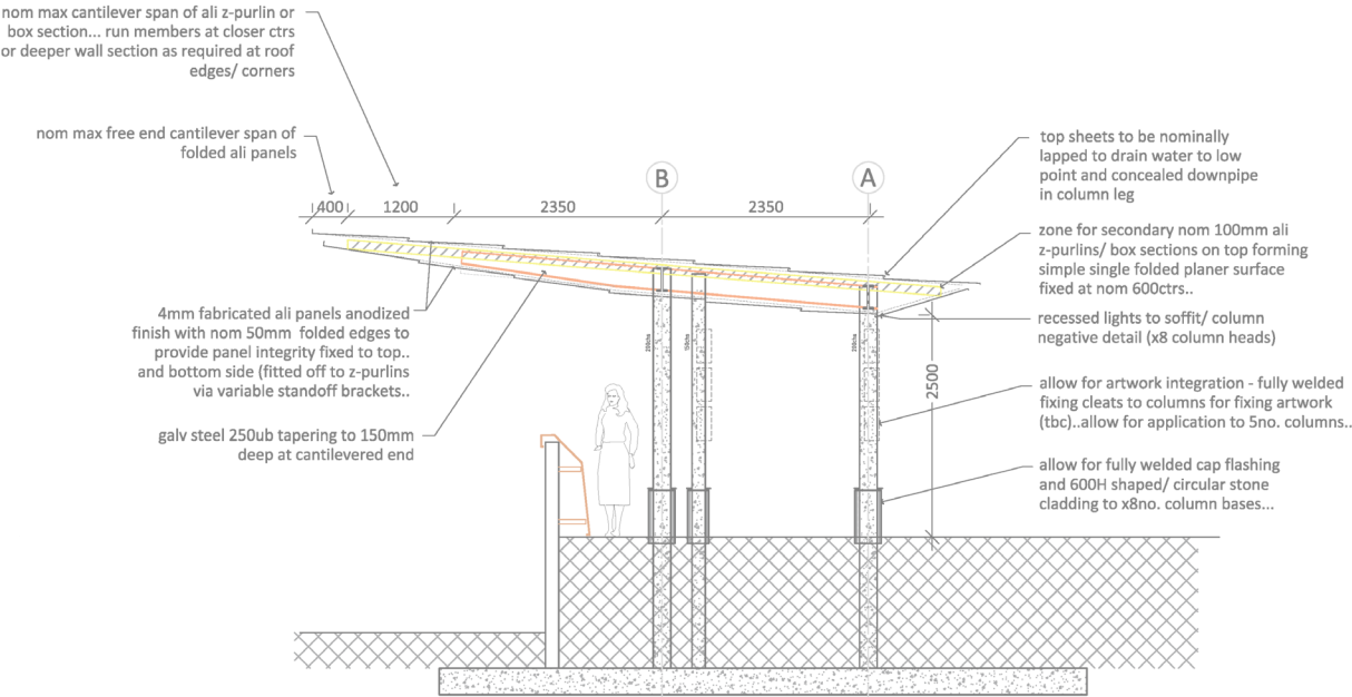
PAVILION 1 SECTION THROUGH GRID 2 LOOKING SOUTH
