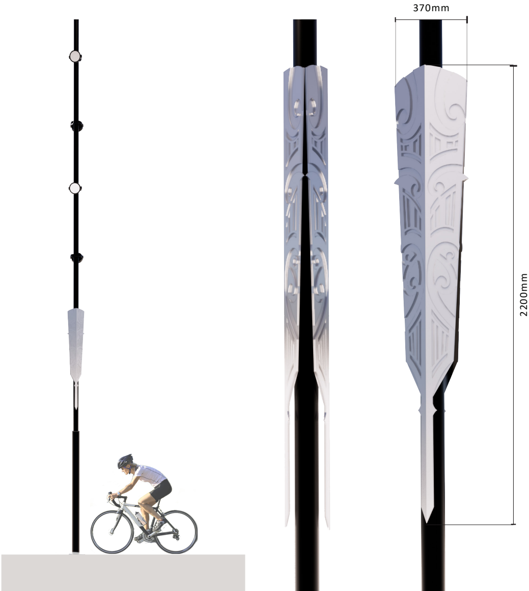
RAUKURA SCULPTURE LIGHTPOLE WRAPS (2B) ● INDICATIVE DESIGN TO BE FURTHER DEVELOPED
