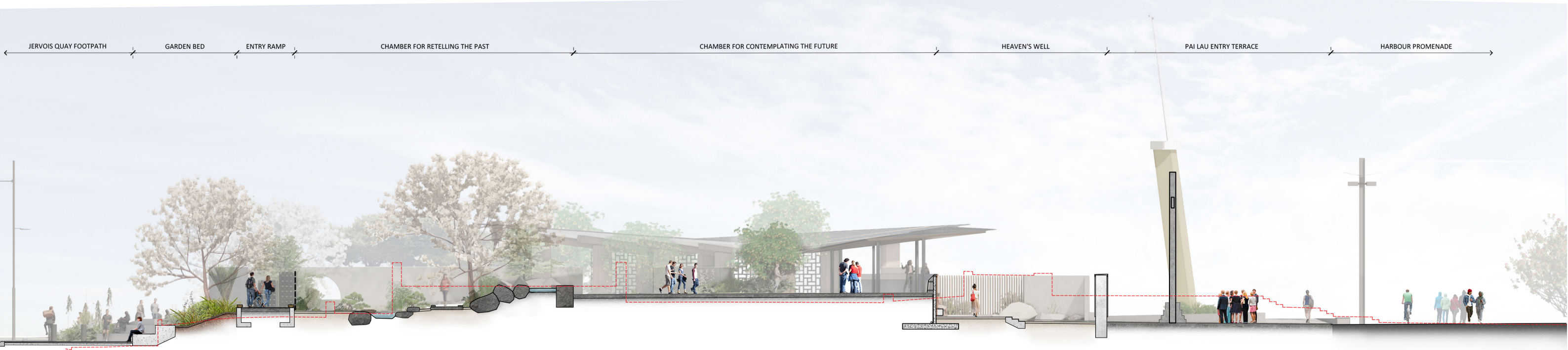
SECTION 2 (S2) - GARDEN OF BENEFICENCE 1:200 @ A3
